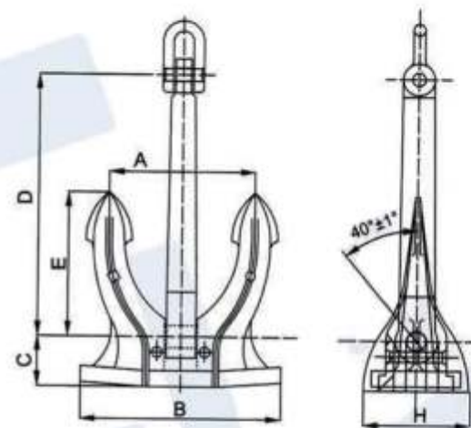
TYPE M SPEK ANCHOR
