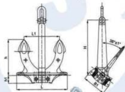
Type B Hall Anchor
