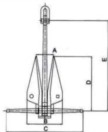
Danforth HHP ANCHOR
