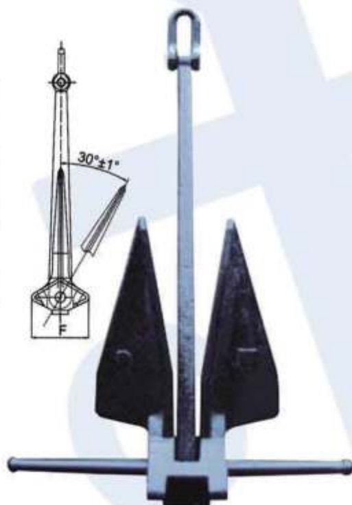
Danforth HHP ANCHOR
