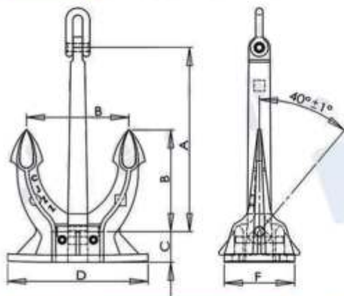
CB711-95 SPEK ANCHOR
